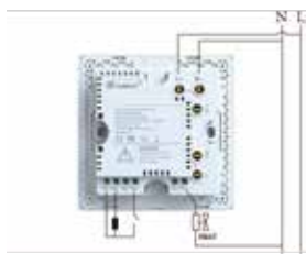
Connection 6: Underfloor heating
