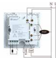
Connection 7: Water source heat pump
